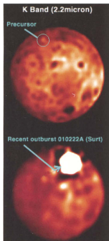
Infrared images collected two days apart, showing the beginning (upper) of the Surt eruption (lower).
