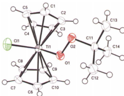
The titanium peroxide complex 1 .
