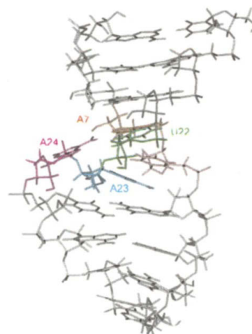
The extruded adenosine (A24) in a \psi -modified duplex.
