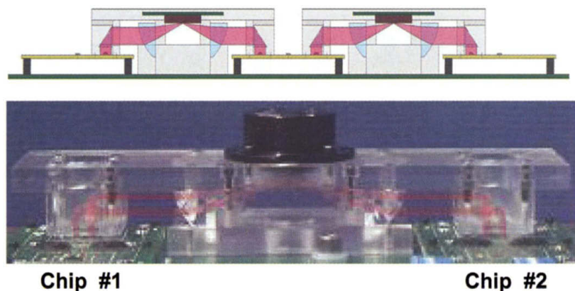
Fig. 5. Chip-to-chip interconnection. Four free-space optical interconnect modules are used to interconnect five daughter boards to accelerate fast Fourier transform calculations on a board. Light from an array of 4 by 4 vertical cavity surface-emitting lasers on each daughterboard exit vertically, are collimated by a lenslet array, and are reflected 90°. The light is then focused by a lens on an adjustable mirror that relaxes the alignment tolerances. A second lens and a lenslet array are used to image the optical signals on a detector array. Use of these modules with 4 by 4 channels operating at 1 Gb/s has been demonstrated with only passive alignment (22).
