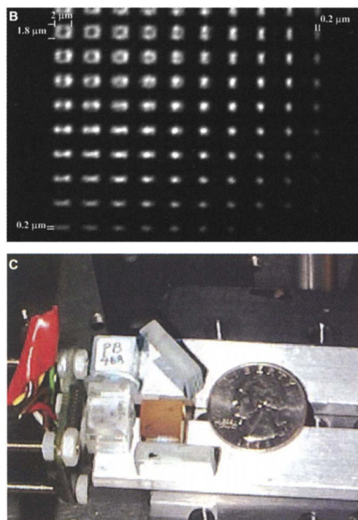
Fig. 6. Holographic memory. (A) Recording is achieved by interfering data recorded on a spatial light modulator and a reference wave. Conventional reconstruction uses the recording reference beam and a lens. Phase-conjugate readout with a counter-propagating reference beam allows lens-less readout. (B) Phase-conjugate readout allows high-density storage. Feature sizes well below 1 \mu\text{m} are visible in the reconstruction shown in (B). One hundred such holograms were superimposed in this experiment, yielding a surface storage density in excess of 100 bits/ \mu\text{m}^2 . (C) Photograph of the experimental apparatus.
