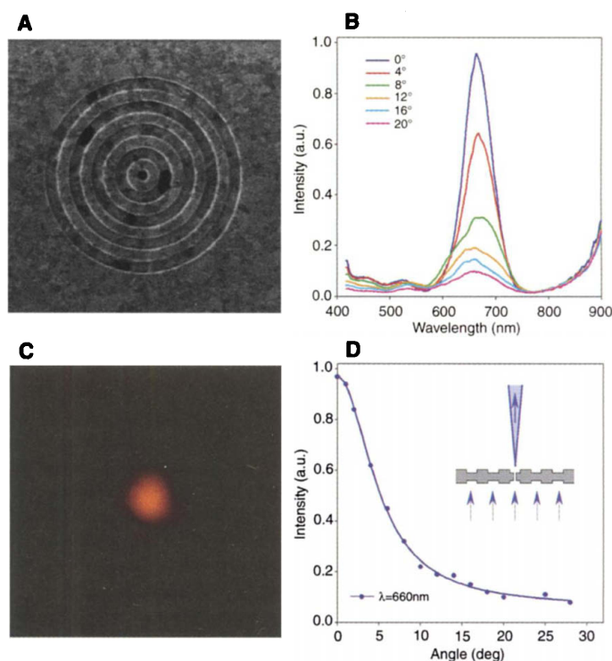
Fig. 1. (A) FIB micrograph image of a bull's eye structure surrounding a cylindrical hole in a suspended Ag film (groove periodicity, 500 nm; groove depth, 60 nm; hole diameter, 250 nm; film thickness, 300 nm). (B) Transmission spectra recorded at various collection angles for a bull's eye structure on both sides of a suspended Ag film (groove periodicity, 600 nm; groove depth, 60 nm; hole diameter, 300 nm; film thickness, 300 nm). The tail above 800 nm is an artifact of the spectral measurement. The structure is illuminated at normal incidence with unpolarized collimated light. The spectra were measured using a Nikon TE200 microscope coupled to an Acton monochromator and a Princeton Instruments CCD (charge-coupled device) camera. (C) Optical image of the sample of (A) illuminated from the back at its wavelength of peak transmission ( \lambda_{\text{max}} = 660 nm) using a 50-nm band-pass filter. (D) Angular transmission-intensity distribution derived from the spectra of (B) at \lambda_{\text{max}} . (Inset) Schematic diagram of the structure and the beam divergence and directionality of the transmitted light at \lambda_{\text{max}} in the far field.
