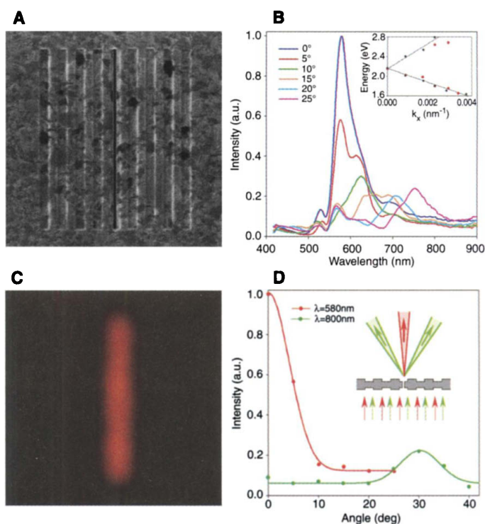
Fig. 2. (A) FIB micrograph image of a slit aperture with parallel grooves on both sides of a suspended Ag film (slit width, 40\ \text{nm} ; slit length, 4400\ \text{nm} ; groove periodicity, 500\ \text{nm} ; groove depth, 60\ \text{nm} ; film thickness, 300\ \text{nm} ). (B) Transmission spectra of the structure of (A) recorded at various collection angles. Illumination at normal incidence with light polarized perpendicular to the slit-length direction. The spectra were measured as in Fig. 1B. (Inset) Dispersion curve (black dots) of the periodic structure as well as the position of the spectral peaks (red dots), plotted as a function of collection angle. (C) Optical image of the sample of (A) illuminated from the back at its wavelength of peak transmission in the forward direction ( \lambda_{\text{max}} = 580\ \text{nm} ) using a 50\text{-nm} band-pass filter. (D) Angular transmission-intensity distribution derived from the spectra of (B) at two selected wavelengths. (Inset) Schematic diagram of the structure showing the corresponding dependence of the directionality on wavelength and the beam divergence in the far field.
