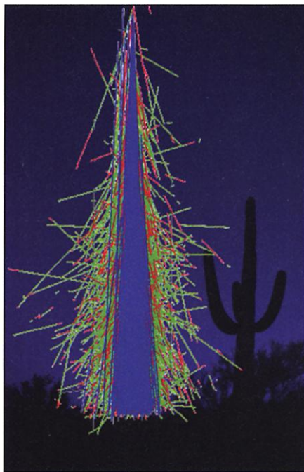
Air show. The most powerful cosmic rays spark cascades of billions of particles.
