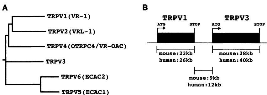
Fig. 1. TRPV3 sequence and genomic localization. (A) Rooted tree showing protein sequence relationship of different members of the TRPV ion channel family. (B) Relative position of TRPV1 and TRPV3 coding sequences on mouse (11B4) and human (17p13) chromosomes.
