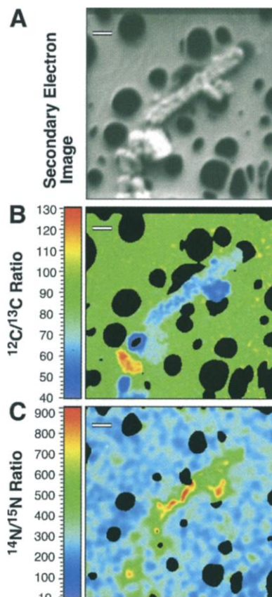
Fig. 4. NanoSIMS (A) secondary electron image and (B and C) isotopic ratio maps of ^{12}\text{C}/^{13}\text{C} and ^{14}\text{N}/^{15}\text{N} , respectively, for the presolar 2H \alpha -SiC shown in Fig. 3. Scale bar, 1 \mu\text{m} .
