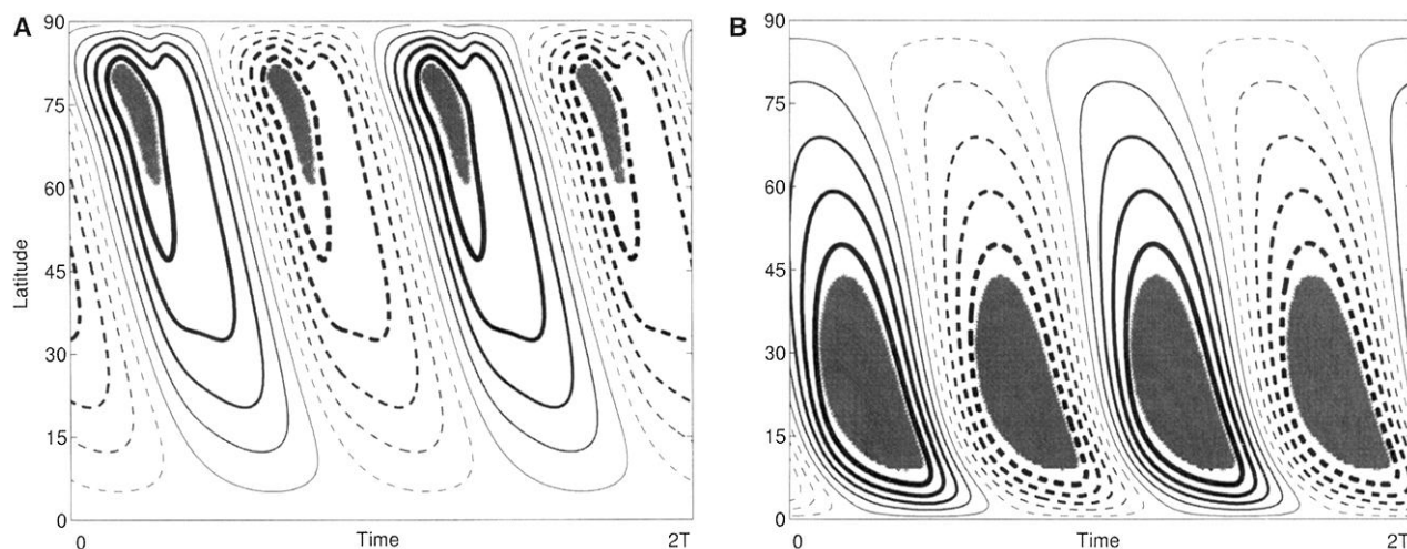
Fig. 2. An eruption latitude versus time plot of sunspots is traditionally called a butterfly diagram. To compare with observations, we construct theoretical butterfly diagrams showing the values of the toroidal magnetic field at the base of the SCZ (at 0.71R ) over two dynamo periods T (equivalent to four sunspot cycles). Solid and dashed contours represent positive and negative values of the magnetic field, respectively, with thicker contours depicting stronger fields. A buoyancy formulation (16, 22) is built into the model, wherein toroidal magnetic fields exceeding 10^5 G above the base of the convection zone (but not below) erupt radially outward to the surface, simulating sunspot formation. Overlaid on the magnetic field contours are gray regions denoting the latitudes at
