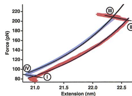
Fig. 4. Experimental realization of the single-molecule operating cycle with polyazopeptides. Five 420-nm flashes drive the polymer into its extended (mainly trans) state (I) at low force (here, 100 pN), and it is then further stretched (red trace). In the stretched state (II), at which a mechanical force F = 200 pN acts on the extended polymer, three 365-nm pulses were applied, which shortens the molecule (trans-cis transition). The force increases during the transition to the shortened state, as an effect of the cantilever stiffness (dotted line), to point III. Upon release of the mechanical stress, the polymer follows the blue trace to point IV, from which a new cycle can be started by switching the shortened configuration to the extended state. The black lines are extended WLC fits, which give contour lengths of 24.8 and 24.5 nm, respectively.
