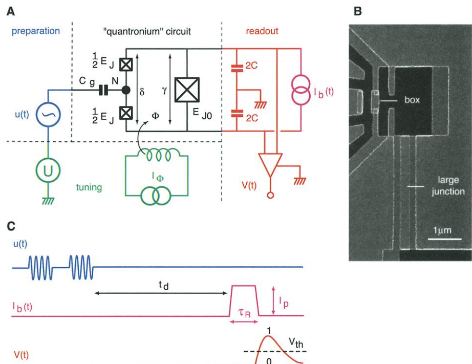
Fig. 1. (A) Idealized circuit diagram of the quantonium, a quantum-coherent circuit with its tuning, preparation, and readout blocks. The circuit consists of a Cooper pair box island (black node) delimited by two small Josephson junctions (crossed boxes) in a superconducting loop. The loop also includes a third, much larger Josephson junction shunted by a capacitance C . The Josephson energies of the box and the large junction are E_J and E_{J0} . The Cooper pair number N and the phases \delta and \gamma are the degrees of freedom of the circuit. A dc voltage U applied to the gate capacitance C_g and a dc current I_\Phi applied to a coil producing a flux \Phi in the circuit loop tune the quantum energy levels. Microwave pulses u(t) applied to the gate prepare arbitrary quantum states of the circuit. The states are read out by applying a current pulse I_b(t) to the large junction and by monitoring the voltage V(t) across it. (B) Scanning electron micrograph of a sample. (C) Signals involved in quantum state manipulation and measurement. Top: Microwave voltage pulses u(t) are applied to the gate for state manipulation. Middle: A readout current pulse I_b(t) with amplitude I_p is applied to the large junction t_d after the last microwave pulse. Bottom: Voltage V(t) across the junction. The occurrence of a pulse depends on the occupation probabilities of the energy eigenstates. A discriminator with threshold V_{th} converts V(t) into a boolean output for statistical analysis.
