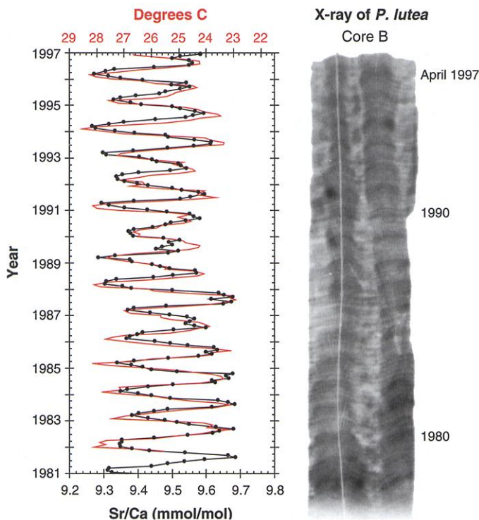
A strong correlation. (Left) Comparison of monthly sea surface temperature (red) for the grid including Rarotonga ( 1^\circ by 1^\circ ; centered at 22^\circ\text{S} , 160^\circ\text{W} ) and Sr/Ca measurements (black) analyzed at 1 mm intervals in a coral core (right) from a colony of P. lutea from Rarotonga.
