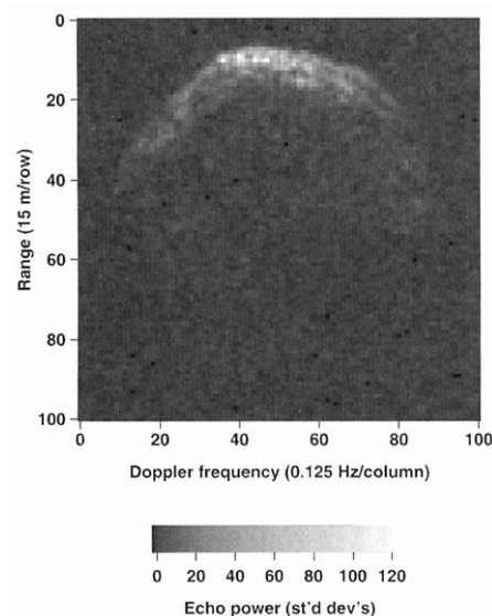
Fig. 1. Arecibo (2380 MHz, 13 cm) delay-Doppler echo-power image of 1950 DA on 4 March 2001, from a distance of 0.052 AU (22 lunar distances). Vertical resolution is 15 m, and horizontal resolution is 0.125 Hz (7.9 mm s -1 in radial velocity).
