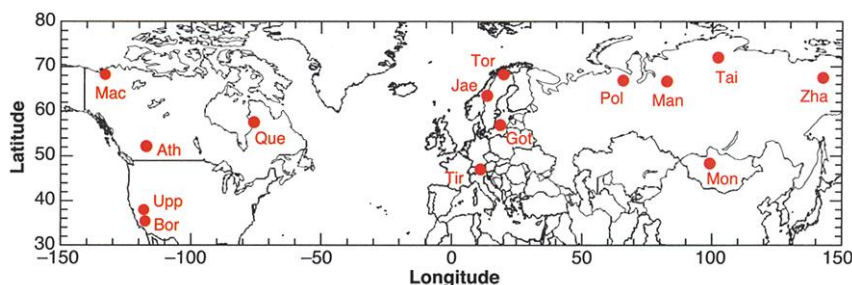
Fig. 1. Map of the 14 tree ring sampling sites. Ath, Athabasca; Bor, Boreal; Mac, Mackenzie; Que, Quebec; Upp, Upperwright; Got, Gotland; Jae, Jaemtland; Tir, Tiro; Tor, Torneträsk; Man, Man; Mon, Mongolia; Pol, Polar Urals; Tai, Taimir; and Zha, Zhaschiviersk.
