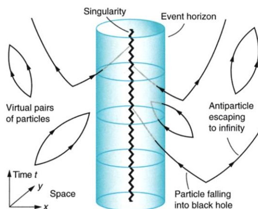
Escape from a black hole. Hawking's most famous discovery was that pairs of particles are created near a black hole. One member falls inside and the other escapes to infinity as Hawking radiation.
