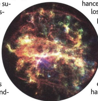
Energies of x-rays emitted by G292.0+1.8 (red, low; blue, high).
