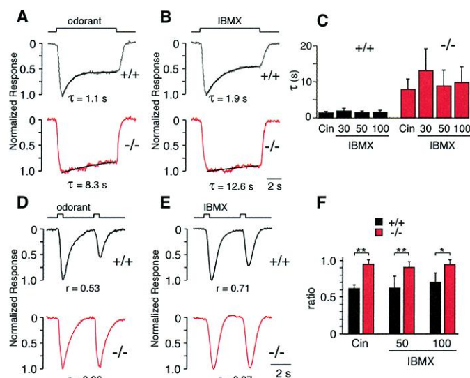
Fig. 2. CNGA4 -/- olfactory receptor neurons exhibit a defect in adaptation. (A and B) Representative EOG responses to an 8-s pulse of (A) cineole or (B) IBMX. 100 \mu M cineole was used to stimulate both +/+ and -/- OE, whereas 50 \mu M and 100 \mu M IBMX were used for +/+ and -/- OE, respectively. At these stimulus concentrations, none of the responses reached saturation. Fits are single-exponential decays with the indicated time constants. (C) Histograms showing collected results (mean \pm SD) from +/+ and -/- mice. Three +/+ animals were treated with the following: cineole, time constant ( \tau ) = 1.4 \pm 0.4 s (100 \mu M, 10 independent measurements); IBMX, \tau = 1.9 \pm 0.7 s (30 \mu M, three independent measurements), 1.5 \pm 0.4 s (50 \mu M, 11 independent measurements) and 1.6 \pm 0.5 s (100 \mu M, three independent measurements), respectively. \tau is significantly increased in the -/- OE [Fisher's least significant difference (LSD) test: P < 0.0001 ]. Five -/- animals were treated with the following: cineole, \tau = 7.9 \pm 2.9 \mu M s (seven independent measurements); IBMX, \tau = 13.1 \pm 6.1 s (30 \mu M, three independent measurements), 8.8 \pm 4.4 s (50 \mu M, nine independent measurements) and 9.8 \pm 4.4 s (100 \mu M, 10), respectively. (D and E) Representative EOG responses to paired 500-ms pulses of (D) cineole or (E) IBMX, delivered with a 3-s interstimulus interval. 100 \mu M cineole was used to stimulate both +/+ and -/- ORNs, whereas 50 \mu M and 100 \mu M IBMX was used for +/+ and -/- animals, respectively. The peak amplitude ratio ( r ) between the first and second responses is indicated at the bottom of each panel. (F) Collected results on the peak amplitude ratio, all measured at a 3-s interstimulus interval. For treatment with cineole, r = 0.62 \pm 0.05 (mean \pm SD, n = 3) for +/+ and 0.95 \pm 0.06 ( n = 5) for -/- mice; **P < 0.0001 , Fisher's LSD test. For treatment with 50 \mu M IBMX, r = 0.62 \pm 0.17 ( n = 4) for +/+ and 0.91 \pm 0.07 ( n = 8) for -/- mice; **P < 0.0001 . For treatment with 100 \mu M IBMX, r = 0.7 \pm 0.13 ( n = 3) for +/+ and 0.94 \pm 0.07 ( n = 7) for -/- mice; *P < 0.001 .
