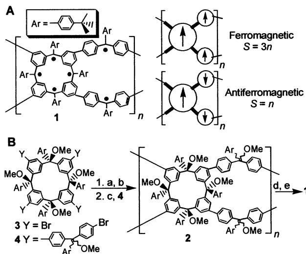
Fig. 1. (A) Polymer 1 with ferromagnetic or antiferromagnetic coupling between the macrocyclic S = 2 and cross-linking S = 1/2 modules. (B) Synthesis of polyether 2 and polymer 1. Reagents: (a) t -BuLi, THF, 198 K (2 hours), 253 K (15 min); (b) \text{ZnCl}_2 , from 198 K to ambient temperature; (c) \text{Pd}(\text{PPh}_3)_4 (3 mol % per CC bond), THF, 373 K (10 min to 5 hours); (d) Na/K, 15-crown-5, THF- d_8 , 283 K (several days); and (e) I_2 , 167 to 170 K.
