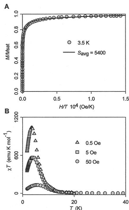
Fig. 2. (A) Magnetic field ( H ) dependence of the magnetization ( M ) of polymer 1 at T = 3.5 K, plotted as M/M_{\text{sat}} versus H/T , where M_{\text{sat}} = 0.54 \mu_B is M at saturation. The solid line corresponds to the least-squares fit using linear combination of Langevin and Brillouin functions corresponding to average S = 5400 (19). (B) Plot of \chi T versus T (dc susceptibility, \chi = M/H ).
