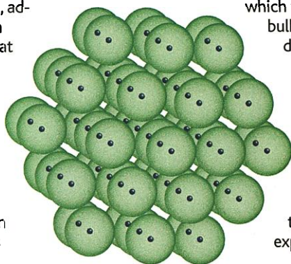
A nearly spherical 59-molecule SF 6 cluster.
