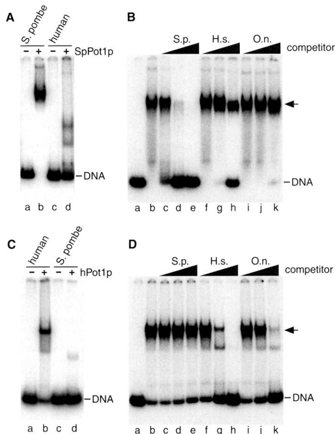
Fig. 5. Substrate specificity of S. pombe and human Pot1p. (A) Binding of SpPot1p to S. pombe and human G-strands (DNA sequences as in Fig. 4). (B) Binding reactions (10 \mu l) contained SpPot1p (50 ng) and radiolabeled S. pombe G-strand (15 pg; GGTACACGGTTAC-AGTTACAGGTTAC-AG) in the presence of 10-, 100-, and 1000-fold excess of unlabeled S. pombe (G-strand sequence as in Fig. 4A), human (TTAGGG) n , or O. nova (GGGGTTT-TGGGGTTT-TGGGGT) DNA. (C) Binding of hPot1p to S. pombe and human G-strands. (D) Binding of hPot1p to human G-strand under the same conditions as in (B).
