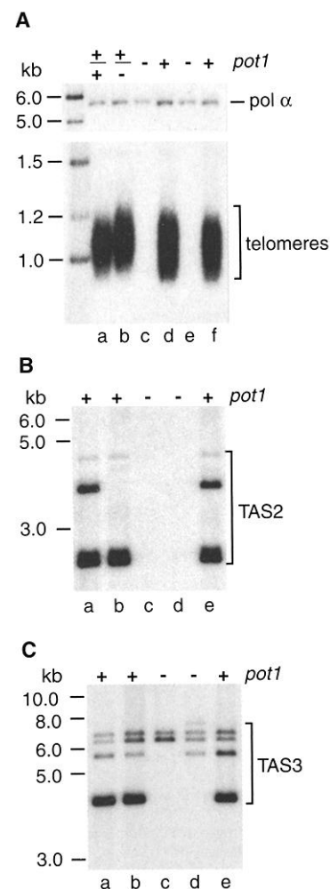
Fig. 2. Telomere phenotype in pot1 − strains. (A) Colonies from the indicated strains were used to inoculate 10 ml of YES (yeast extract supplemented with amino acids) medium at 32°C. Cells were grown to late log phase, and genomic DNA was prepared. After digestion of DNA (~20 \mu g) with Eco RI, samples were subjected to 1.1% agarose gel electrophoresis, transferred to a nylon membrane, and hybridized to a telomeric probe. As a loading control, a probe against the single-copy pol \alpha gene was used. (B) Genomic DNA (~20 \mu g) was digested with Nsi I, fractionated by 0.8% agarose gel electrophoresis, transferred to a nylon membrane, and hybridized to a TAS2 probe (18). (C) The blot in (B) was stripped (34) and hybridized to a TAS3 probe.
