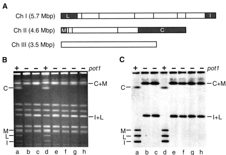
Fig. 3. Pulsed-field gel electrophoresis and detection of terminal fragments. (A) Schematic showing the location of Not I restriction sites on S. pombe chromosomes (47). Only terminal fragments on chromosomes I and II are labeled. (B) Ethidium bromide-stained pulsed-field gel containing Not I-digested DNA from two pot1 + strains and six independent pot1 - isolates. Genomic DNA was prepared, Not I-digested, and fractionated by pulsed-field gel electrophoresis as described (34). (C) DNA from the gel shown in (B) was transferred to a nylon membrane and hybridized to gene-specific probes on the C, I, L, and M fragments.
