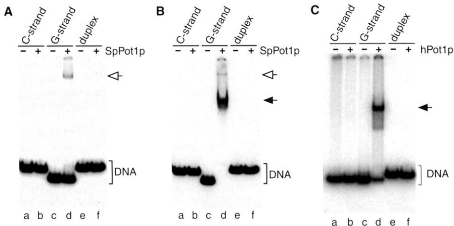
Fig. 4. DNA-binding specificity of SpPot1p. (A) C-strand (CGTAACCGTAACCCGTGAACCTGTAACCTGTAACCGTGAACCC) and G-strand (GGTTACACGGTTACAGGTTACAGGTTACAGGGTTACGTTTACG) were 5' ^{32} P-labeled using T4 polynucleotide kinase and [ \gamma - ^{32} P]adenosine triphosphate. Duplex was generated by annealing equimolar amounts of radiolabeled C-strand and unlabeled G-strand. Pot1p (50 ng) was incubated with the indicated DNA substrates (1 ng) for 15 min at 20°C in 10 \mu l of 25 mM Hepes (pH 7.5), 1 mM EDTA, 50 mM NaCl, 5% glycerol, and 2.5 \mu M PBol109 (CCGTAAGCATTTTCATTATTGGAATTCGAGCTCGTTCGCA) as nonspecific competitor. Complexes were analyzed by electrophoresis at 4°C through a 4 to 20% tris-borate EDTA gel (Invitrogen) run at 150 V for 80 min. The Pot1p-DNA complex is indicated by an open arrow. (B) Same as (A) except that the added protein (100 ng) contained truncated Pot1p as well as full-length protein. Truncated Pot1p-DNA complex is indicated by a solid arrow. (C) Binding of hPot1p to human C-strand (CCCTAA) n , G-strand (TTAGGG) n , and duplex DNA.
