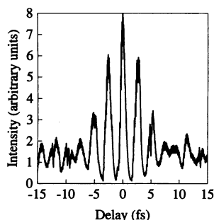
Fig. 1. Second-order interferometric autocorrelation trace of the 5-fs laser pulses used in the experiment. The fringe spacing is \approx 2.6 fs, corresponding to the light oscillation cycle at wavelength \lambda = 780 nm.
