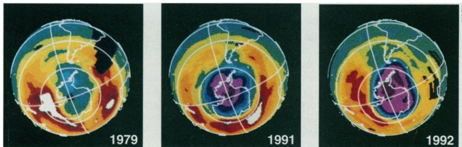
A bigger beast. The Antarctic ozone hole (pink and dark blue) had grown to record size by 23 September of this year—15% larger than ever before, but ozone concentration was above last year's record low.
