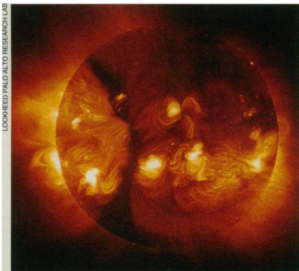
Movie star. Bright "active regions" dot the sun in this still from an x-ray motion picture of the solar corona.
