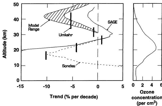
Fig. 9. Comparison of ozone profile trend estimates from several measurement systems, SAGE, Umkehr, and ozonesonde stations. SAGE data are an average of the latitudes 50°N and 50°S. The Umkehr is the average over five northern mid-latitude stations. The ozonesondes are an average over six northern mid-latitude stations. Shaded area shows the range of two model calculations at 50°N and 50°S. The panel on the right shows a typical ozone concentration versus altitude.
