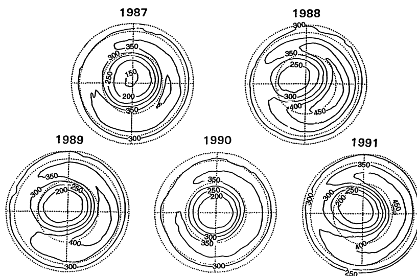
Fig. 1. Polar orthographic projections of TOMS Southern Hemisphere maps of October mean total ozone for each of the last 5 years. The South Pole is at the center; the equator, 30°S, and 60°S latitude circles are shown; and Greenwich is to the top. The contours are in Dobson units.
