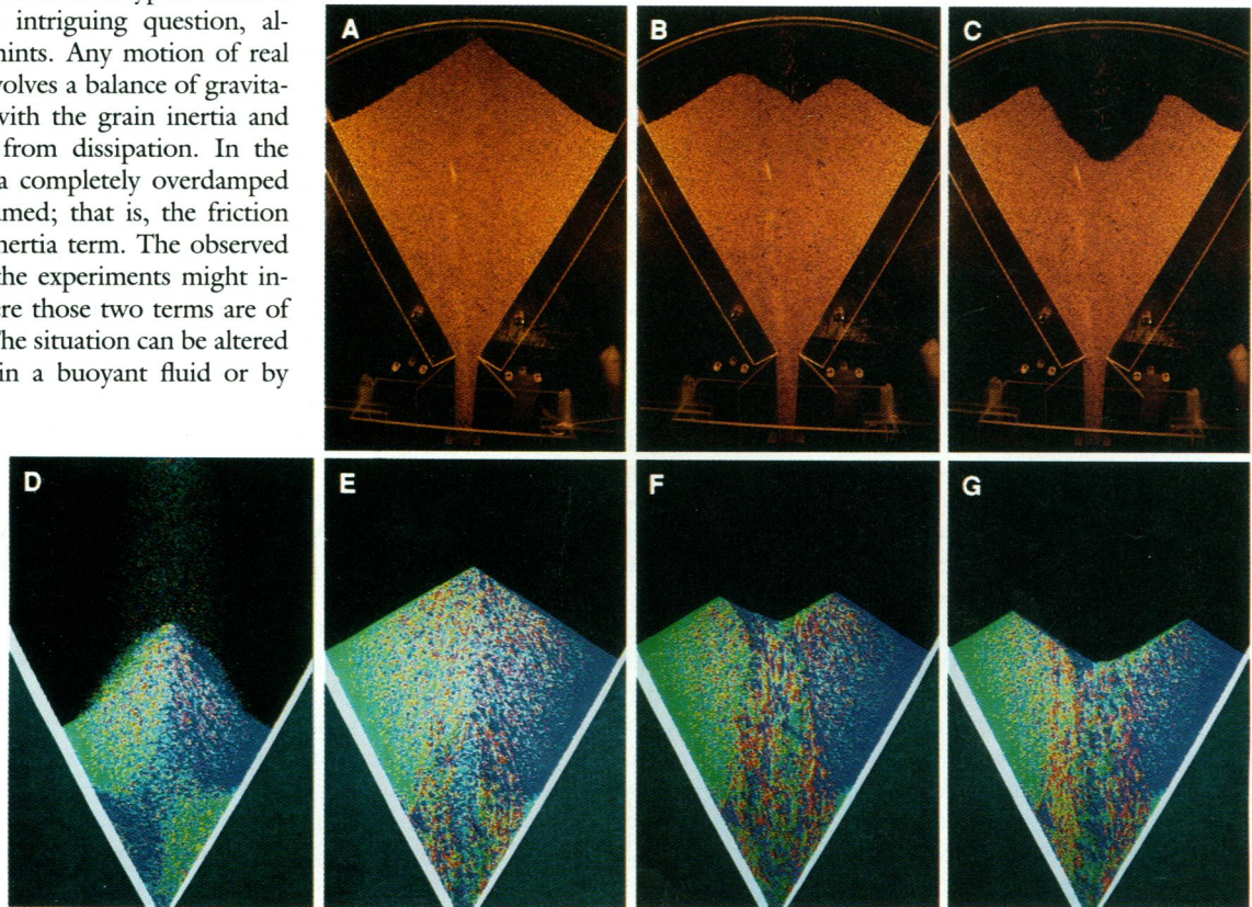
Fig. 3. Photographs of grass seed flowing through a hopper (A) immediately, (B) 0.6 s, and (C) 2.6 s after the opening of the aperture. The grass seeds rapidly align along the direction of the flow. (D through G) Cellular automata simulations on a triangular lattice of the same process. For each site a velocity and orientation is assigned. The particle can either be at rest or can move with velocity \pm|v| along any of the three lattice directions. The orientation can likewise be along any of the three lattice directions. The colors indicate the orientation of the “seeds” (blue, inclined to the left; green, inclined to the right; red, vertical). The images show (D) the filling process, in which particles are added from the top with random orientations (the “crosslike” green and blue background pattern in the hopper is caused during the early stages of the filling
