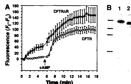
Fig. 1. (A) Fluorescence of SPQ-loaded HeLa cells (13) expressing CFTR (○) ( n = 17 , where n = number of cells) or CFTR \Delta R (●) ( n = 5 ). \text{NO}_3^- was substituted for \text{I}^- in the bathing medium at 0 min. Five minutes later (arrow) cells were stimulated with 20 \mu\text{M} forskolin and 100 \mu\text{M} IBMX (cAMP). Data are mean \pm SEM. Without addition of forskolin and IBMX the fluorescence did not increase further after 5 min in either group. (B) Expression of CFTR and CFTR \Delta R in transfected HeLa cells. Cells were transfected with pTM-CFTR4 (lane 1) or pTM-CFTR4 \Delta R (lane 2) (12). Twelve hours after transfection, cells were incubated with [ ^{35}\text{S} ]methionine (25 \mu\text{Ci}/\text{ml} ) for 1 hour and lysed in 50 mM Tris (pH 7.5), 150 mM NaCl, aprotinin (100 \mu\text{g}/\text{ml} ), 0.1 mM phenylmethylsulfonyl fluoride, and 1% digitonin (250 \mu\text{l} per 35-mm dish). CFTR and CFTR \Delta R were immunoprecipitated from cell lysates with a monoclonal antibody to a synthetic peptide from the COOH-terminus of CFTR (amino acids 1466 to 1480) (26). Immunoprecipitates (50 \mu\text{l} per lane) were analyzed by SDS-polyacrylamide gel electrophoresis and autoradiography. Molecular weight standards are 170, 94, 67, and 43 kD.
