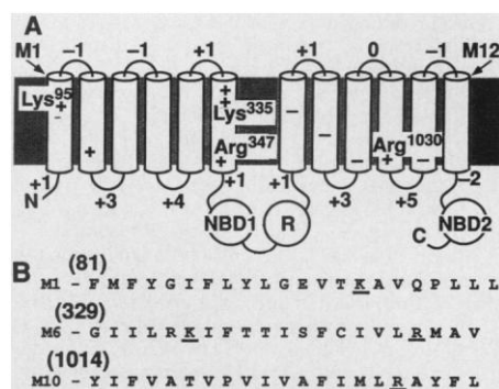
Fig. 1. Predicted topology of CFTR in the membrane. (A) M1 to M12, membrane-spanning sequences; NBD1 and NBD2, nucleotide-binding domains; R, regulatory domain. Charged residues in M1 to M12 are indicated by + and -. Predicted net charges of intracellular and extracellular loops are indicated; charge of first five amino acids only, before M1 and M7 and after M6 and M12, are indicated. (B) Sequences of M1, M6, and M10. Amino acids mutated in this study are underlined. The single-letter code for the amino acids is as follows: A, Ala; R, Arg; D, Asp; C, Cys; Q, Gln; E, Glu; G, Gly; I, Ile; L, Leu; K, Lys; M, Met; F, Phe; P, Pro; S, Ser; T, Thr; Y, Tyr; V, Val.
