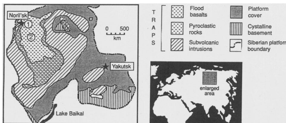
Fig. 1. Geologic sketch map of part of the Siberian platform showing the distribution of the Siberian Traps [after (11)]. Circled numbers indicate locations of the Noril'sk (1) and Putorana (2) sections.
