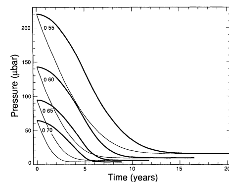
Fig. 2. Response of Triton's atmospheric pressure to a change in bolometric bond albedo from 0.74 to 0.85. The heavy curves are for a linear change in albedo over a period of 5 years, and the light curves are for an instantaneous change. Curve pairs are plotted for several different emissivities, ranging from 0.55 for the top pair to 0.70 for the bottom pair in steps of 0.05. A combined contribution of 6 mW m^{-2} from internal heat flow and absorbed thermal energy from Neptune has been included, chosen so that, for an emissivity of 0.55, the final equilibrium pressure is 15 \mu bar.
