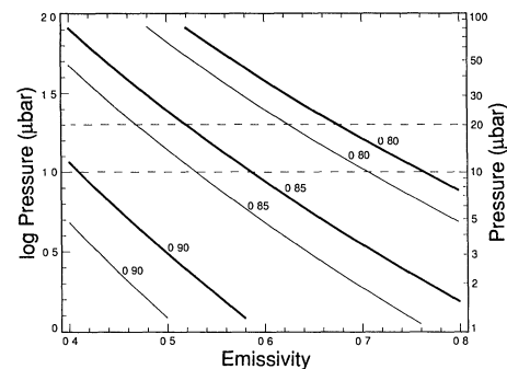
Fig. 1. Triton's surface pressure as a function of emissivity for three values of bolometric bond albedo. The heavy line is for a model that includes solar, internal radiogenic, and Neptune energy inputs. The light line is for a model that includes only solar input, and the area between the dashed, horizontal lines is the range of pressure 15 \pm 5 \mu bar, encompassing the range of Voyager measurements of Triton's surface pressure (2). Radiogenic heat and heat from Neptune in this model amount to 6 mW m^{-2} .
