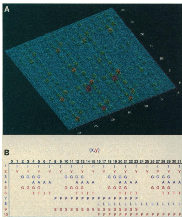
Fig. 7. (a) Fluorescence scan of an array of 1024 peptides generated by a ten-step binary synthesis. Following photochemical and side group deprotection, the array was treated with antibody 3E7 and then fluorescein-labeled antibody as described in the preceding legends. The polynomial expression for this ten-step binary synthesis is
