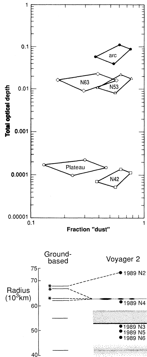
Fig. 21. This figure shows the radial locations of the most reliable ground-based occultation detections of material around Neptune compared against the locations of ring material as seen in Voyager imaging data. Asterisks denote ground-based observations confirmed by more than one telescope.
