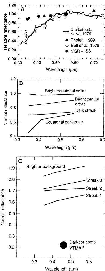
Fig. 27. Triton colors and albedos. (A) Ground-based spectra of Triton in the visual and near infrared taken in 1979 as well as contemporaneously with the Voyager encounter of Neptune are shown (64, 65). Plotted with the ground-based data are the Triton disk-averaged colors as obtained from Voyager narrow-angle camera images. Note the substantial color change from 1979 to 1989 shown by these data. (B) Normal reflectance of selected areas on the encounter hemisphere of Triton are shown (see text). (C) Normal reflectances of selected dark areas on Triton are shown. The brighter background spectrum is an average of bright areas adjacent to the dark streaks whose normal albedos are also plotted. The darkest spot is located north of the equator in the darker, redder plains.
