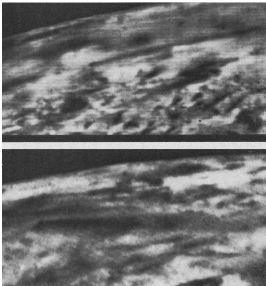
Fig. 38. Profile view of Triton's active geyser-like plumes. These two high-emission-angle views are of the regions near the southern limb; south is up, west to the right. In both views the spacecraft was about 15^\circ above the horizon as seen from the base of each plume near its source. The plumes are about 8 km tall; the east-west dimension of the two views is about 150 km. The west plume is shown in top image; the east plume in the bottom image.
