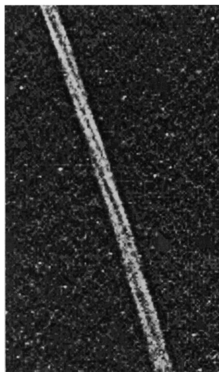
Fig. 18. This narrow angle, clear filter image (FDS 11412.46) was part of the outbound (high phase angle) retargetable sequence along with Fig. 14 and shows a portion of the trailing arc. The sky plane resolution is about 14 km per line pair and the phase angle is about 135^\circ . The combination of uncompensated spacecraft motion and ring orbital motion causes points to streak in the image. However, the width and separation of the streaks reveal the scale size and longitudinal distribution of clumps in the rings. In addition to the fine scale information revealed in the streaked clumps, this image seems to show width variations which would imply that the arc may be resolved (see text).
