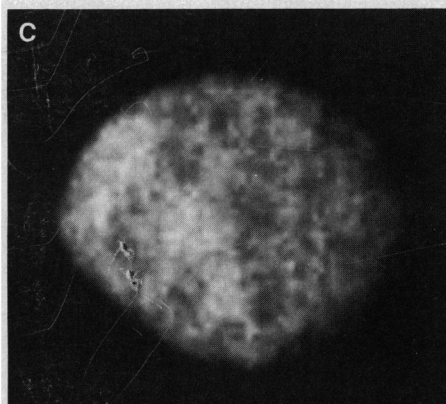
Fig. 39. Voyager 2's best views of 1989N1 and 1989N2. (A) 1989N1 is shown in this image at a resolution of 7.9 km per pixel; (B) 1989N1 is at 1.3 km per pixel; and (C) 1989N2 at 4.2 km per pixel. (D) Schematic of the viewing geometry. Arrows labeled S/C indicate spacecraft view; letters correspond to images A, B, and C.
