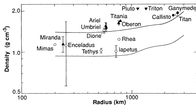
Fig. 22. Comparison of radius and observed mean density for outer solar system objects. Filled circles are satellites of Jupiter, open circles satellites of Saturn, triangles satellites of Uranus, and inverted triangles Pluto and Triton. The upper curve represents a simple compression model for a satellite with 60% water ice and 40% silicate (53); the lower curve is a pure water-ice model for comparison.
