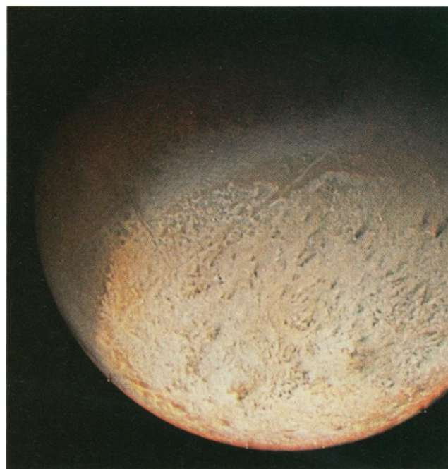
Fig. 28. Color image of Triton acquired at a range of 530,000 km with a resolution of 10 km per line pair. Narrow angle images obtained with green, violet, and ultraviolet filters were used as the red, green, and blue components. High frequency information from a clear image, containing the greatest detail, was merged with the color data.
