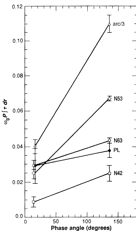
Fig. 19. In this figure, observations of the radially integrated brightness of different regions of the Neptunian rings are shown as functions of phase angle. The brightness has been converted to the "equivalent width" product \omega_0 P f \tau dr , in units of kilometers, where f \tau dr is the "equivalent depth" and \tau is the normal optical depth. The regions are the N42, N53, and N63 rings (not including the ring arcs), the plateau region averaged between 55,000 and 58,000 km, and the middle ring arc (plotted at one-third of its actual values).
