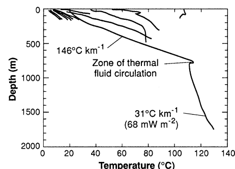
Fig. 4. Temperature-depth profiles from drill holes collared in rocks older than 6 Ma in the Breitenbush Hot Springs area (8, 10, 11). The deepest hole was completed to 2457 m, but was only logged to 1715 m. The bottom-hole (2457 m) temperature was >141^\circ\text{C} (26). The gradient measured over the 1465- to 1715-m interval ( 31^\circ\text{C km}^{-1} ) projects to a bottom-hole temperature of 152^\circ\text{C} .
