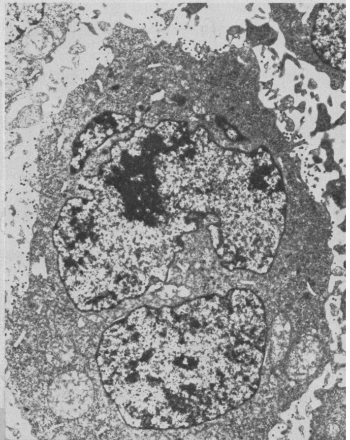
AIDS virus
