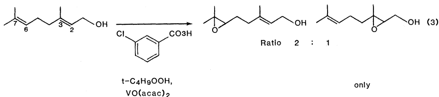
Fig. 1. Chemoselective epoxidation.
