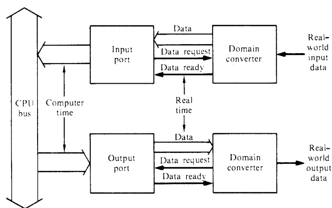
Fig. 2. Parallel I-O interface between the CPU bus and domain converters. The input and output ports connect domain converters appropriate for the real-world devices to the CPU bus. Data transfers are synchronized by the "handshaking" signals Data ready and Data request . [Reprinted with permission from Benjamin/Cummings Publishing Company (2)]
