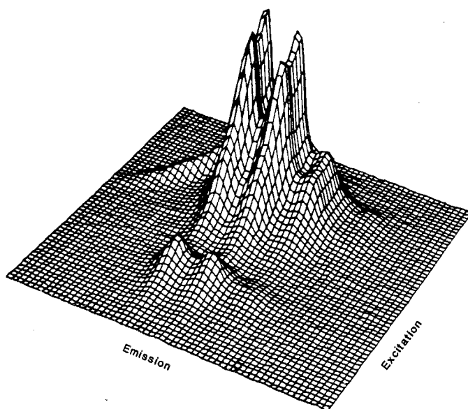
Fig. 3. Three-dimensional projection of an emission-excitation matrix corresponding to the chromatographic peak of benzo[a]pyrene from a sample of shale oil. [From (9)]
