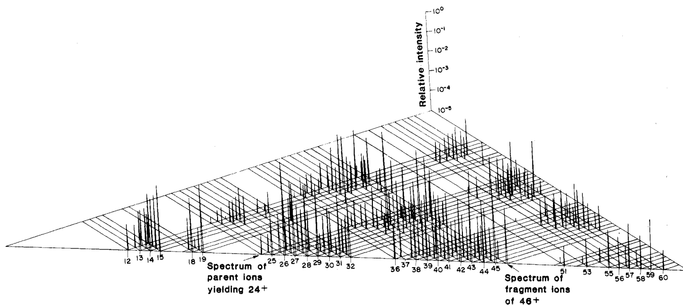
Fig. 5. Three-dimensional projection of the ions observed for all combinations of masses selected by the first and third quadrupoles in the TQMS for a sample of pure isopropanol. Different slices through this data matrix provide different kinds of information about the sample. [From (11)]
