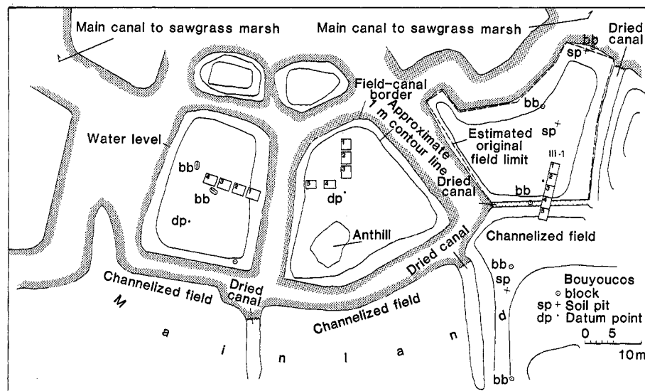
Fig. 5. Aerial plan of raised and channelized fields and canals at raised field site 1, located along the midsection of the western side of the southern arm of Pulltrouser Swamp. The numbered squares are excavation units.
