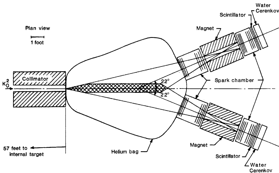
Fig. 1. Plan view of the apparatus as located at the Brookhaven AGS.
