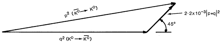
Fig. 4. Vector diagram showing schematically the difference in the amplitudes for K^0 \rightarrow \bar{K}^0 and \bar{K}^0 \rightarrow K^0 .
