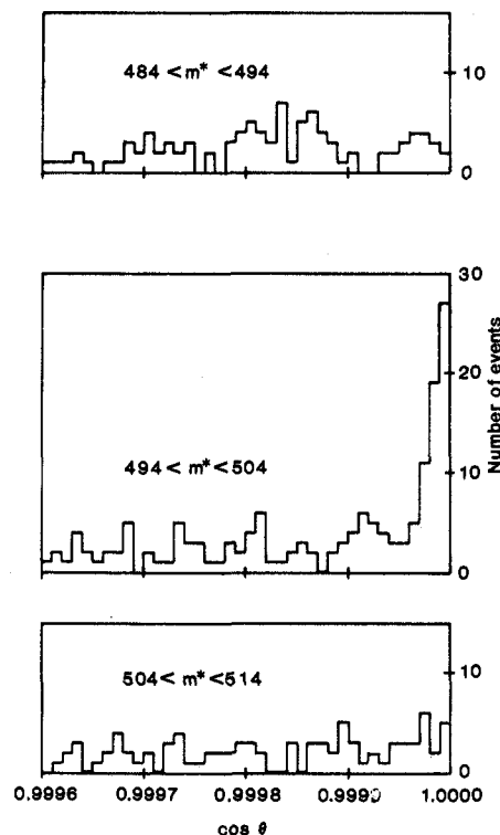
Fig. 3. Angular distribution of the events after measurement by a precise machine in three relevant mass regions.
