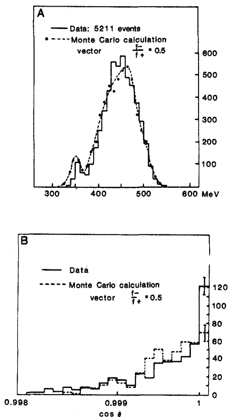
Fig. 2. Angular distribution of the events in the appropriate mass range measured by a coarse machine.
