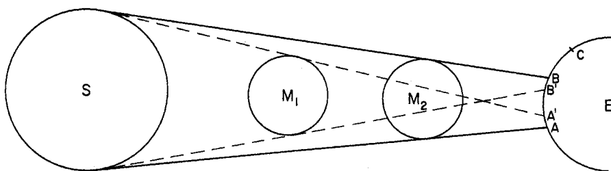
Fig. 1. Geometry of the moon's shadow during solar eclipses. With the moon at M_1 , an observer between A'B' sees an annular eclipse. With the moon at M_2 , an observer between AB sees a total eclipse; at C , a partial eclipse is seen.
