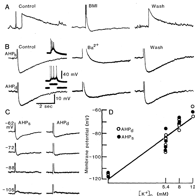
Fig. 2. Ionic mechanism of the AHPs. (A) A CA1 pyramidal cell recorded with a KCl-filled pipette. In the presence of 10^{-4} M pentobarbital, orthodromic stimulation produces a pronounced depolarizing IPSP (control). After the medium is changed to one containing BMI, the response is reversibly replaced by a burst of action potentials and an AHP s ; resting potential, -55 mV. (B) Comparison of the effects of 2 mM Ba 2+ on the AHP s and AHP d in a single cell. In the presence of BMI (Control), both orthodromic (top) and direct (bottom) stimuli produce large AHP's. Twenty-six minutes
