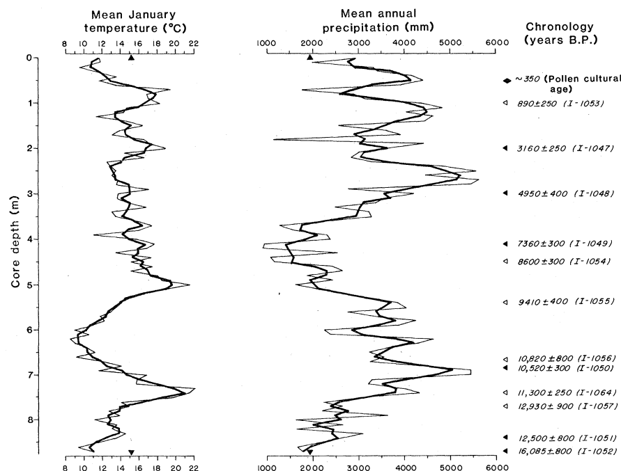
Fig. 2. Mean January temperature and mean annual precipitation for the past 16,000 years at Alerce. Bold lines represent three-point moving averages of the data. The triangles on the temperature and precipitation scales denote modern mean values, closed triangles on the right denote ^{14}\text{C} -dated levels in the Alerce core, and open triangles denote ages from nearby sites (13) that are pollen-stratigraphically correlated with Alerce.
