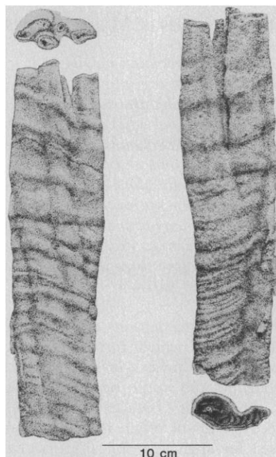
Fig. 2. Sketches of a portion of a flattened compound tube showing simple upward branching and preservation of bedding structures.
