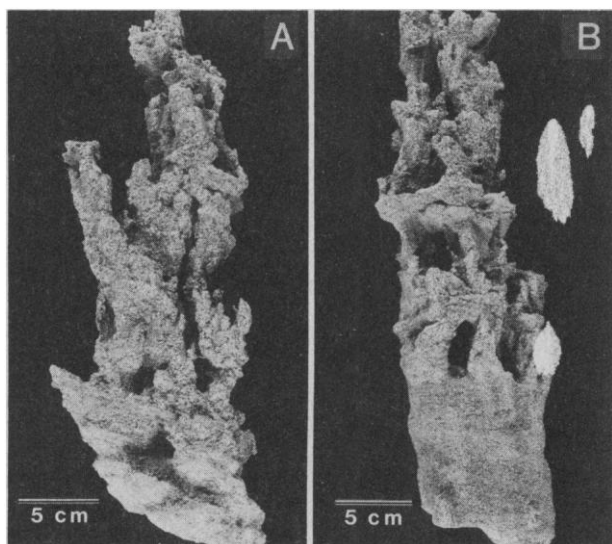
Fig. 4. Arborescent sand columns.
