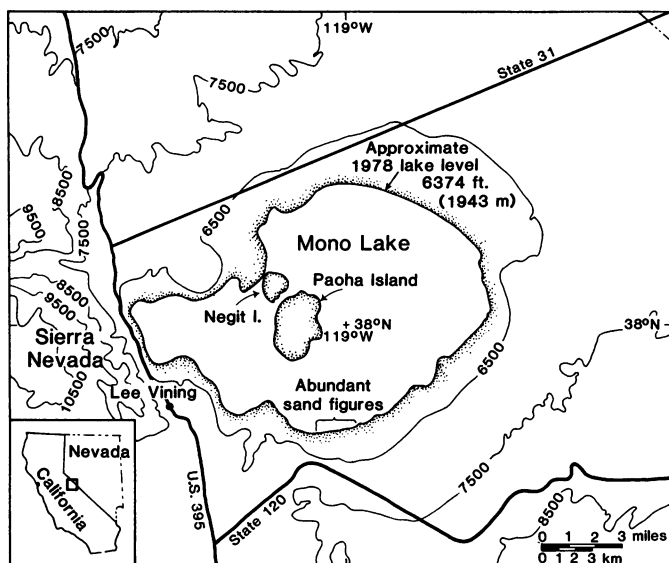
Fig. 1. Index map of Mono Lake area. Contour elevations are in feet (after USGS (topographic map)).
