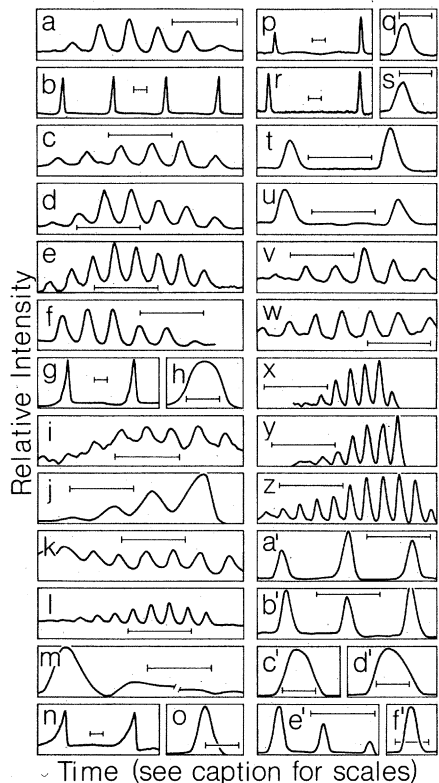
Fig. 1. Chart traces of flash patterns of flying male fireflies. The bars represent 0.25 second, except h, o, q, s, c', d', and f', where the bars represent 0.125 second (all are single, simple flashes). Recordings were made in the field with a photomultiplier magnetic-tape system. (a) Pyractomena barberi , 18.3°C (compare c). (b) Photuris VR's own pattern, 15.6°C. (c) Photuris VR flicker, 19.4°C. (d) Pyractomena angulata , 20.0°C (compare e, f, i, k, and l). (e) Photuris B, 23.3°C. (f) Photuris tremulans , 19.4°C. (g) Photuris Mo, 19.7°C. (h) Photuris AR's own pattern, 15.5°C. (i) Photuris Mo, 19.7°C. (j) Photuris CR's own (?) pattern, 18.9°C. (k) Photuris CR, 18.9°C. (l) Photuris cinctipennis , 25.0°C. (m) Photuris pennsylvanica 's own pattern, 13.6°C. (n) Photuris cinctipennis ' (Florida) own flash, 21.7°C. (o) Pyractomena limbicollis , 18.6°C (compare f'). (p) Photinus macdermotti entire pattern, 22.2°C (compare r), and (q) individual flash at faster chart speed (compare s). (r) Photuris cinctipennis , 22.2°C, and (s) individual flash at faster chart speed. (t) Photinus consanguineus , 23.6°C (compare u). (u) Photuris cinctipennis , 23.6°C. (v) Colombian Photinus sp., 21.9°C (compare w). (w) Colombian Photuris sp., 21.9°C. (x) Photinus evanescens s.l., 21.7°C (compare y). (y) Photuris jamaicensis , 21.7°C. (z) Photinus commissus , 22.2°C. (a') Photinus lineellus , 26.2°C (compare b'). (b') Photuris A, 24.4°C. (c') Photinus curtatus × marginellus , 17.2°C (compare d'). (d') Photuris pennsylvanica , 13.6°C. (e') Photuris versicolor 's (Florida) own pattern, 21.7°C. (f') Photuris versicolor (21.7°C). Patterns paired here for demonstration were selected for clarity of form and, therefore, temperatures are sometimes not matched.
