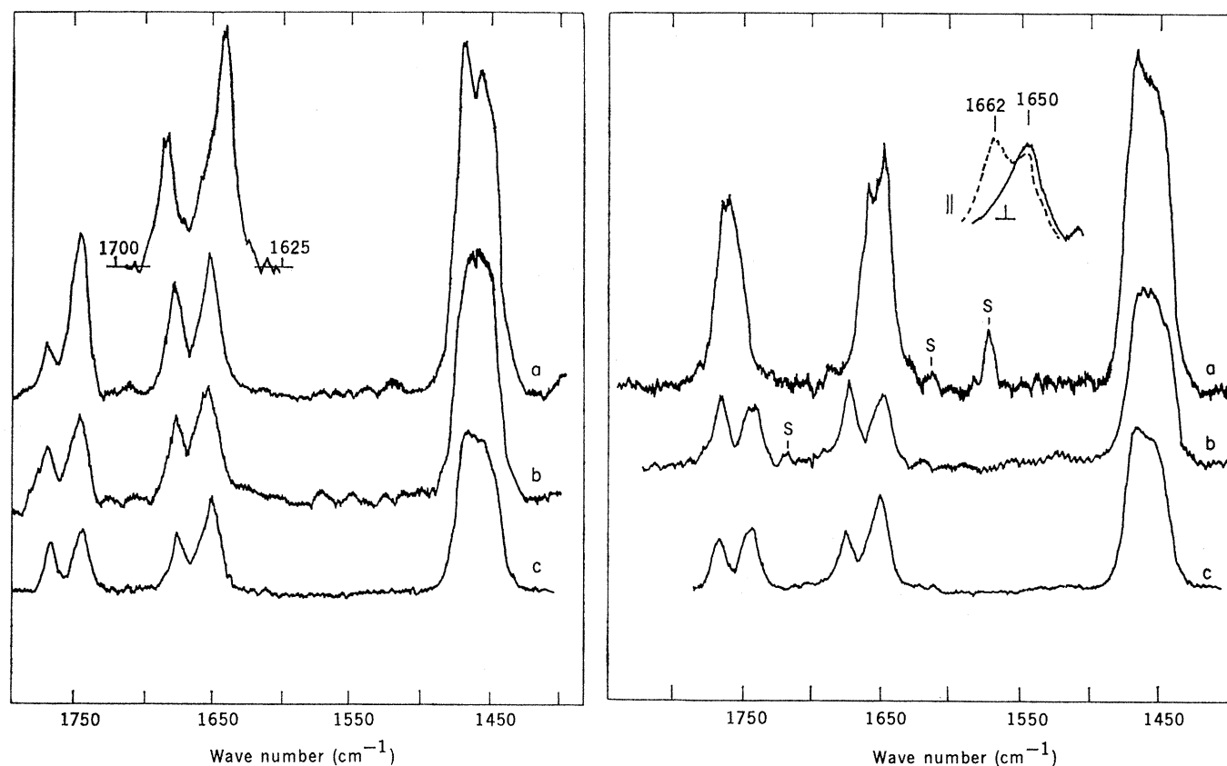
Fig. 2 (left). Raman spectra of valinomycin grown from octane. Spectra were obtained at a scanning speed of 20\text{ cm}^{-1}/\text{min} and a slit width of 4\text{ cm}^{-1} . (a) Crystal; incident light ( 5208\text{ \AA} ) polarized perpendicular to the plane of scattering. (b) Crystal; incident light ( 5208\text{ \AA} ) polarized parallel to the plane of scattering. (c) Powder; incident light, 5145\text{ \AA} . (Inset) Higher-resolution spectrum of the crystal with incident light ( 4880\text{ \AA} ) polarized parallel to the plane of scattering; scanning speed, 5\text{ cm}^{-1}/\text{min} ; slit width, 2\text{ cm}^{-1} . Fig. 3 (right). Raman spectra, obtained at a scanning speed of 20\text{ cm}^{-1}/\text{min} and a slit width of 4\text{ cm}^{-1} , of (a) valinomycin crystal grown from o -dichlorobenzene ( 5145\text{ \AA} ); (b) valinomycin crystal grown from acetone ( 4880\text{ \AA} ); (c) valinomycin powder from octane ( 5145\text{ \AA} ). (Inset) Effect of rotating the polarization of the incident light on the amide I peaks of valinomycin crystals grown from o -dichlorobenzene. The symbols are: S, solvent peaks; \perp , light perpendicular to the scattering plane; \parallel , light parallel to the scattering plane. The scanning speed was 10\text{ cm}^{-1}/\text{min} and the slit width 2\text{ cm}^{-1} .
