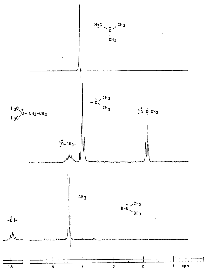
Fig. 1. The PNMNMR spectra of the t -butyl cation (top), t -amyl cation (middle), and isopropyl cation (bottom). Note large deshielding effects and the long-range coupling in the t -amyl cation indicating sp^3 \rightarrow sp^2 rehybridization at the potential carbonium ion center.
