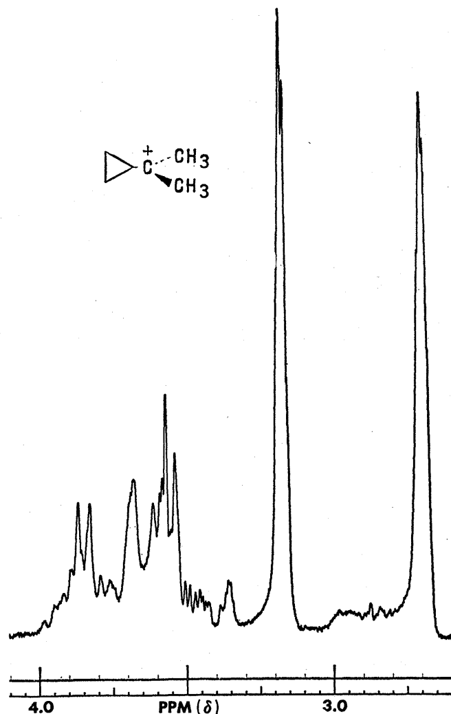
Fig. 2. The PNMR spectrum of the dimethylcyclopropyl carbonium ion shows nonequivalent methyl group proving the "bisected" structure.
