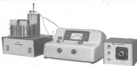
Automatic Sampling Assembly consisting of Thomas 20-tube Roto-Sampler with Suction Pump and Flow Control Timer; for completely automatic transfer of samples to Spectronic 20 Spectrophotometer
