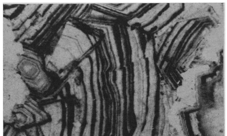
Fig. 1 (above left). Calcite infilling in dolomite. The top photograph was taken by luminescence from the specimen only. The bottom photograph is of the same region of the same specimen, taken with crossed Nicols. All the luminescence photographs are negatives. The dark areas correspond to bright luminescence and the light areas to dim luminescence. Fig. 2 (above right). Calcite infilling in dolomite. A region as photographed by luminescence (top) and with crossed Nicols (bottom). Fig. 3 (below left). Calcite infilling in dolomite. A region as photographed by luminescence (top) and with crossed Nicols (bottom). Fig. 4 (below right). Calcite infilling in dolomite. This photograph was taken by luminescent light, using higher magnification. Under the microscope this single grain revealed 50 distinguishable growth bands.
