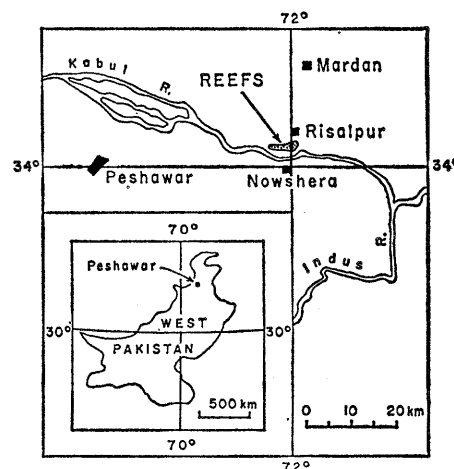
Fig. 1. Paleozoic reefs in Pakistan.
