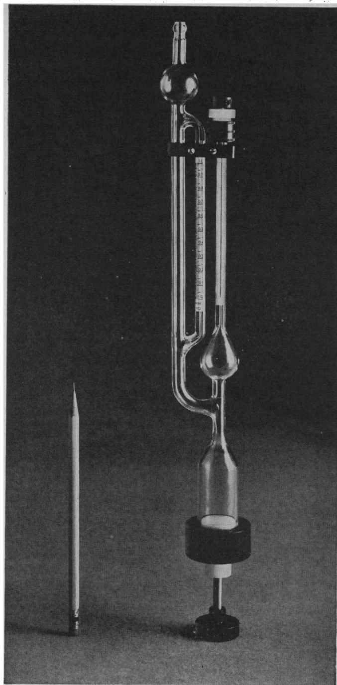
Simple, compact new McLeod Gage with adjustable closed end
