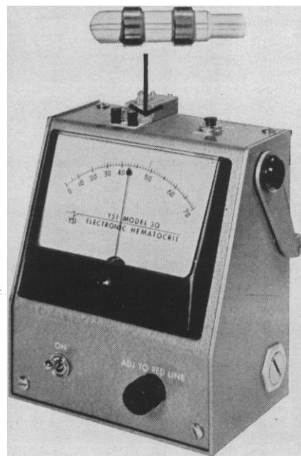
YSI Model 30
