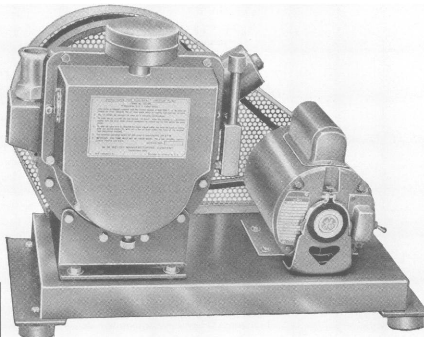
Illustration Shows 1397-B Duo-Seal ® Pump Equipped With Vented Exhaust
