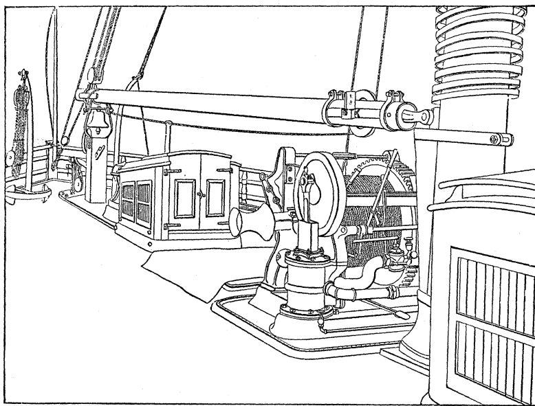
FIG. 4.—THE FORWARD DECK OF THE U. S. FISH-COMMISSION STEAMER FISH HAWK, LOOKING FORWARD FROM THE PILOT-HOUSE, SHOWING THE HOISTING AND REELING ENGINE AND THE DREDGING-BOOM.
