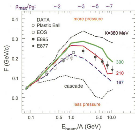
Fig. 2. Transverse flow results. The solid and open points show experimental values for the transverse flow as a function of the incident energy per nucleon. The labels “Plastic Ball,” “EOS,” “E877,” and “E895” denote data taken from Gustafsson et al. (13), Partlan et al. (14), Barrette et al. (15), and Liu et al. (16), respectively. The various lines are the transport theory predictions for the transverse flow discussed in the text. \rho_{\text{max}} is the typical maximum density achieved in simulations at the respective energy.
