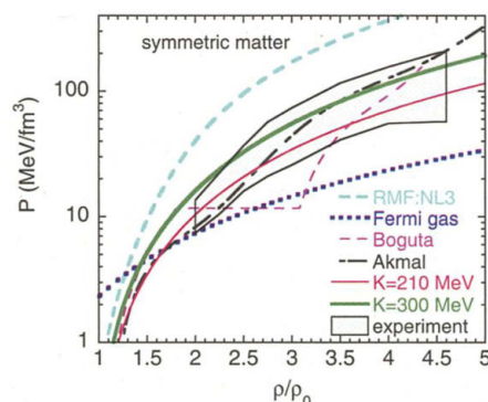
Fig. 3. Zero-temperature EOS for symmetric nuclear matter. The shaded region corresponds to the region of pressures consistent with the experimental flow data. The various curves and lines show predictions for different symmetric matter EOSs discussed in the text.
