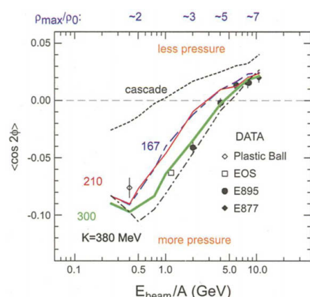
Fig. 4. Elliptical flow results. The solid and open points show experimental values for the elliptical flow as a function of the incident energy per nucleon. The labels “Plastic Ball,” “EOS,” “E895,” and “E877” denote the data of Gutbrod et al. (17), Pinkenburg et al. (18), Pinkenburg et al. (18), and Braun-Munzinger and Stachel (19), respectively. The various lines are the transport theory predictions for the elliptical flow discussed in the text.
