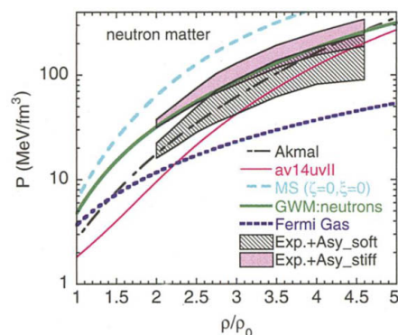
Fig. 5. Zero-temperature EOS for neutron matter. The upper and lower shaded regions correspond to the pressure regions for neutron matter consistent with the experimental flow data after inclusion of the pressures from asymmetry terms with strong and weak density dependences, respectively. The various curves and lines show EOS predictions for different neutron matter EOSs discussed in the text.
