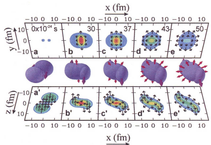
Fig. 1. Overview of the dynamics for a Au + Au collision. Time increases from left to right, the center of mass is at r = 0 , and the orientation of the axes is the same throughout the figure. The trajectories of projectile and target nuclei are displaced relative to a "head-on" collision by an impact parameter of b = 6 \text{ fm} ( 6 \times 10^{-13} \text{ cm} ). The three-dimensional surfaces (middle panel) correspond to contours of a constant density \rho \sim 0.1 \rho_0 . The magenta arrows indicate the initial velocities of the projectile and target (left panel) and the velocities of projectile and target remnants following trajectories that avoid the collision (other panels). The bottom panels show contours of constant density in the reaction plane (the x - z plane). The outer edge corresponds to a density of 0.1 \rho_0 , and the color changes indicate steps in density of 0.5 \rho_0 . The back panels show contours of constant transverse pressure in the x - y plane. The outer edge indicates the edge of the matter distribution, where the pressure is essentially zero, and the color changes indicate steps in pressure of 15 \text{ MeV/fm}^3 ( 1 \text{ MeV/fm}^3 = 1.6 \times 10^{32} \text{ Pa} ; that is, \sim 1.6 \times 10^{27} atmospheres). The black arrows in both the bottom and the back panels indicate the average velocities of nucleons at selected points in the x - z plane and x - y planes, respectively.
