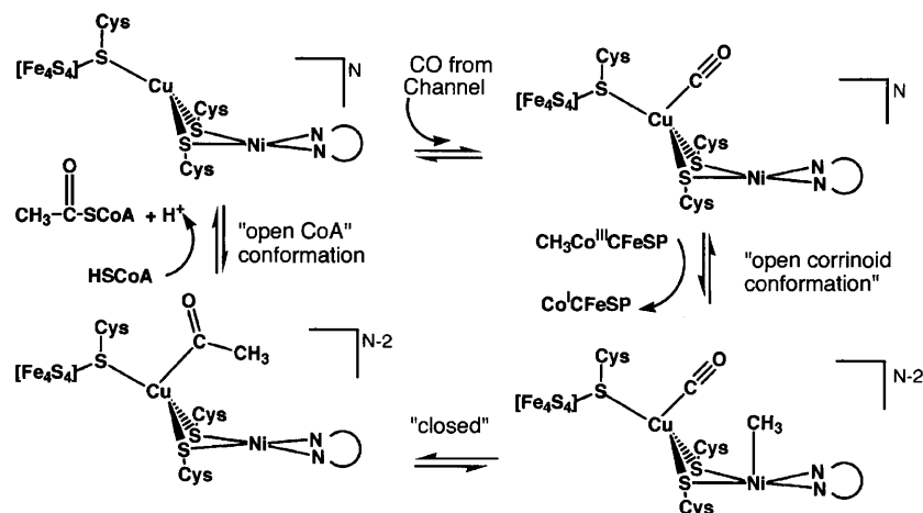
Fig. 3. Simplistic mechanistic proposal for acetyl-CoA synthase activity. Although experimental data indicate that the reaction of an acetyl-metal intermediate with CoA is the last step in the mechanism (7, 20), the data do not distinguish between CO binding and methylation as the first step. In this scenario, we propose that CO generated from CO 2 at the C-cluster travels through the putative channel and binds to Cu. Ni has been proposed to act as a nucleophile attacking the methyl group of protein-bound methylcob(III)amide, resulting in cob(II)amide and a methylated Ni species (14). The reaction of CO and methyl group could proceed through an alkyl migration yielding an acetyl-metal-bound intermediate. In the final step, HSCoA is deprotonated and acetylated. The oxidation states of metals during catalysis are highly controversial (2, 31) and cannot be resolved here. However, the presence of three Cu thiolate ligands suggests that Cu is likely to be in the Cu(I) oxidation state throughout catalysis. The coordination of Ni by two thiolates and two deprotonated peptide nitrogens should favor higher oxidation states of Ni: Ni(II) with no axial ligands and Ni(III) when an axial ligand is bound (44). The presence of the [Fe 4 S 4 ] moiety of the A-cluster close to the surface of the enzyme suggests that oxidation states including all ferrous could be considered for this cubane (45).
