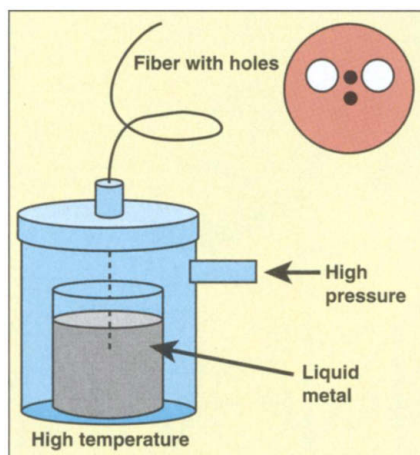
Pressure injection of a liquid alloy at 170°C.
